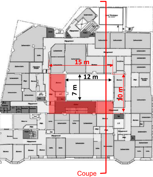
PLAN EXISTANT
